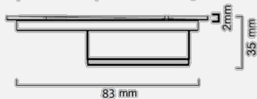
Adaptador PVC (Grelha 10cm / grate 10cm / Rejilla 10cm)
