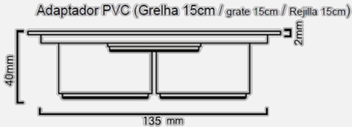
Vista Superior / Top View / Vista Superior
