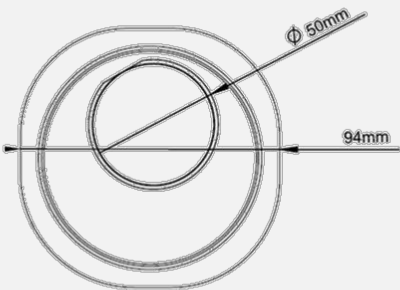
Adaptador PVC (Grelha 10cm / grate 10cm / Rejilla 10cm)
